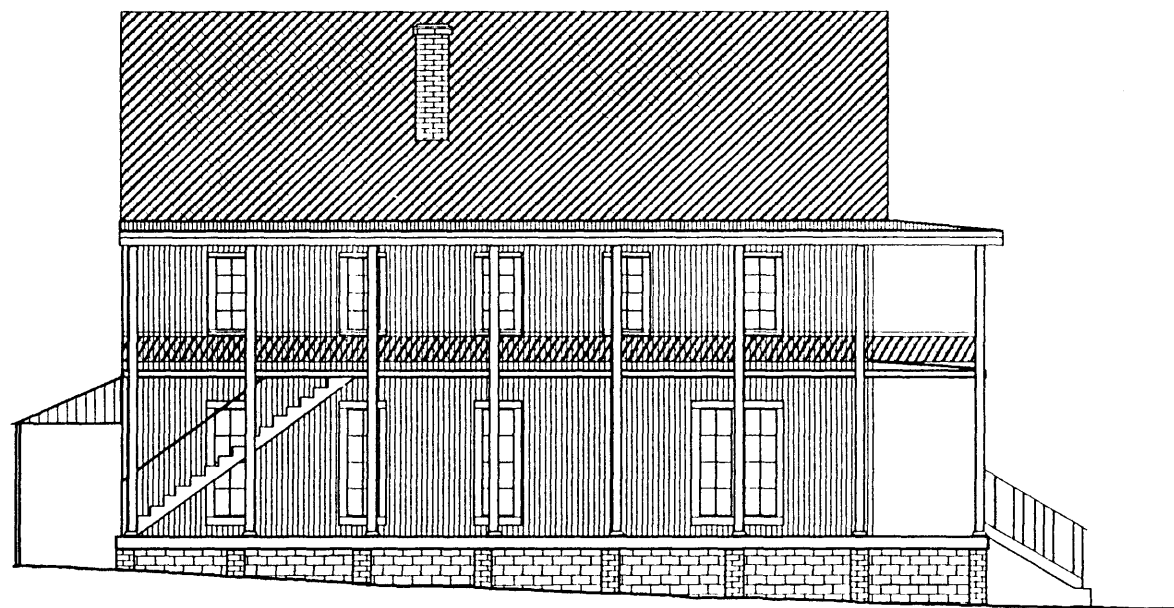
Stafford-Wells North Elevation
